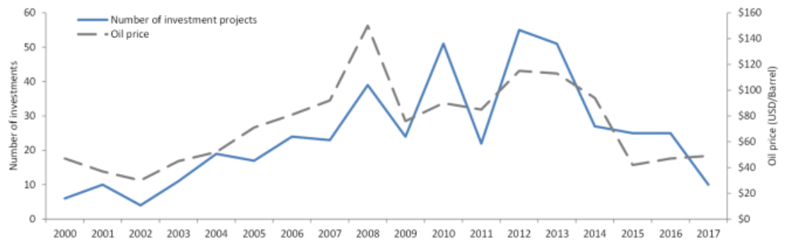
Figure 2 Investments by the Gulf states into the Horn and oil price.
